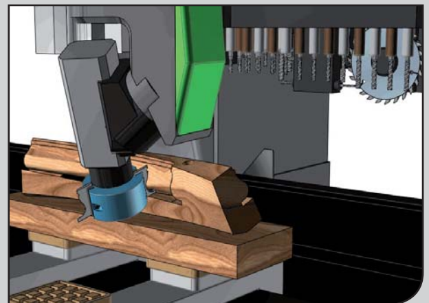
Complex 5 axis machining with TopSolid'WoodCam 2009.
